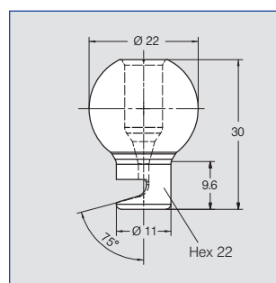
Tongue type nozzle with ball joint, Swivel-mounted 30° in all directions.
