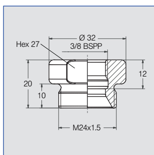
Retaining nut for ball joint Ordering no. 092.020.1E.67.38
