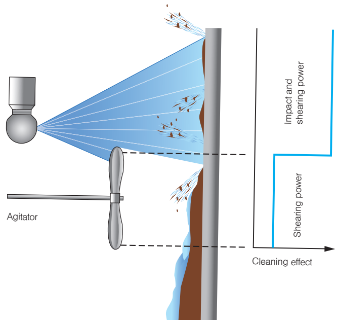
Figure 5: Cleaning mechanisms, impact and shearing power
