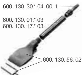
600. 130. 56. 01 with accessories *01 = 1.0711 / 17 = 316 SS / 30 = Brass
