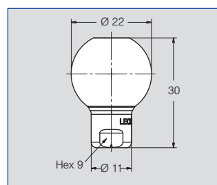
Flat fan nozzle with ball joint, 30° Swivel-mounted 30° in all directions.
