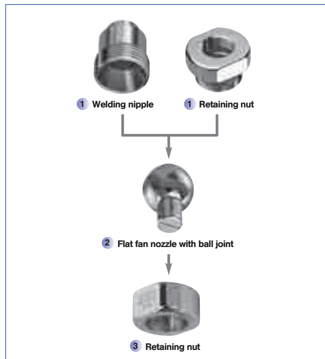
Welding nipple for ball joint Ordering no. 092.020.1E.67.04
