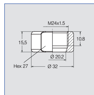
Retaining nut for ball joint Ordering no. 092.020.1E.67.02
