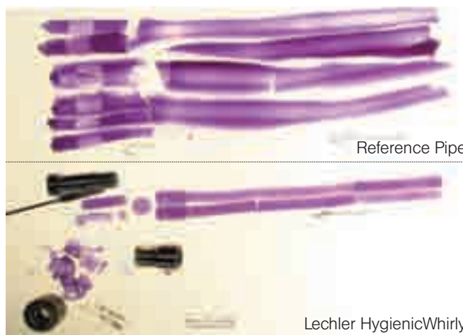
Figure 11: EHEDG In-place Cleanability Test of a Lechler HygienicWhirly. The result shows no differences between the reference pipe and the HygienicWhirly. In both cases the breeding ground is purple, indicating no germ formation
