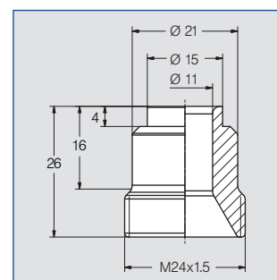
Welding nipple for ball joint Ordering no. 092.020.1E.67.04
